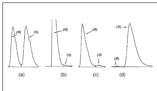
Scheme 3. Chiral-phase GC analysis of α-keto ester reduction products. Samples were analyzed on a 25 m Chirasil-Dex CB column. (a) Racemic 2 prepared by NaBH 4 reduction of 1 . (b) ( R )- 2 prepared by Candida boidinii CIOC21 reduction of 1 in aqueous medium. (c) ( R )- 2 prepared by Candida boidinii CIOC21 reduction of 1 in aqueous medium with 10% (v/v) DMSO as a cosolvent. (d) ( S )- 2 prepared by Yarrowia lipolytica CIOC1502 reduction of 1 .
