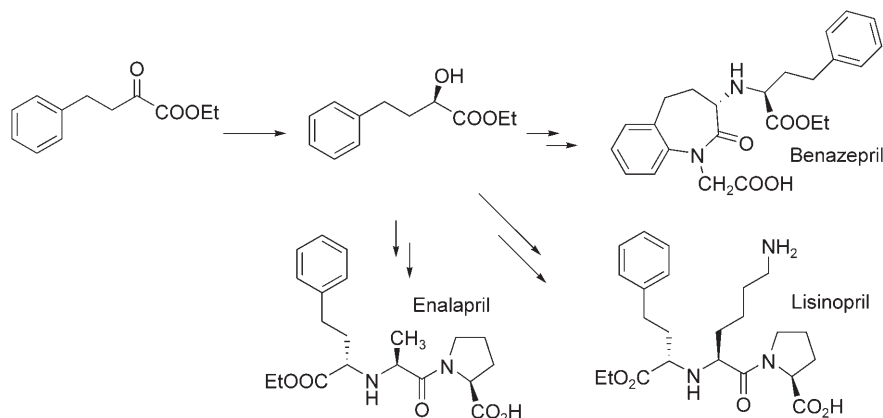
Scheme 1. Process for the production of ACE inhibitors.
