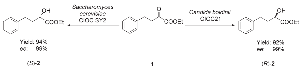
Scheme 2. Stereoselective reduction of keto ester 1 .
